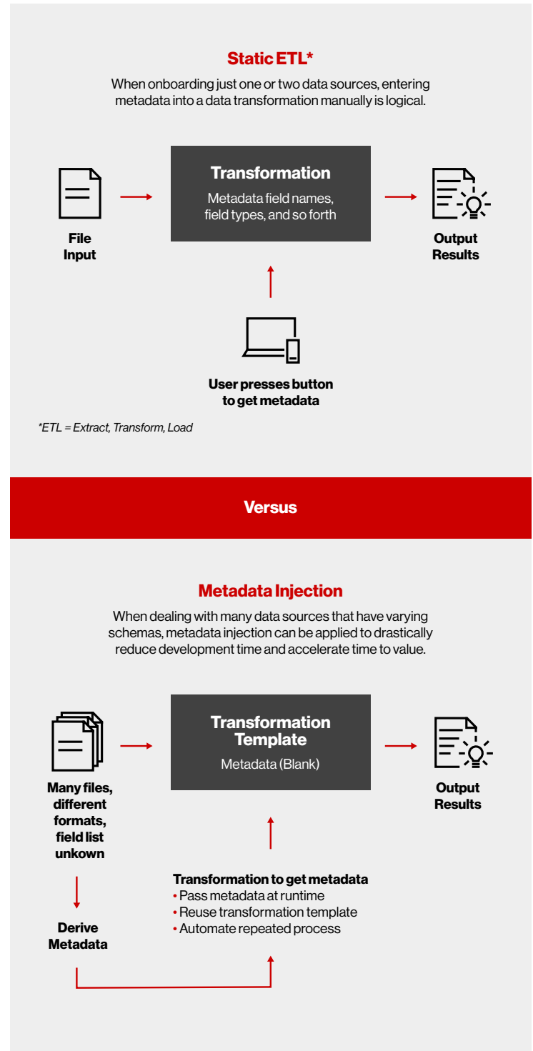
Fig. 1 Compare static ETL with metadata injection for data-onboarding.
